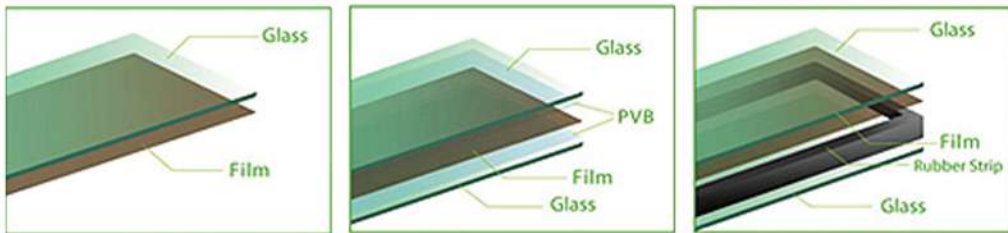
Image 1.1 Privacy Glass Structure
