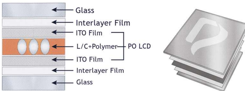
Image 1.2 Privacy Glass™ Structure
